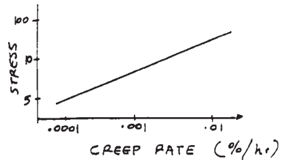
FIG. X3.2 Creep Strength
