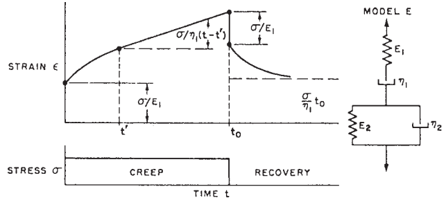
FIG. X6.3 Four Element Model
