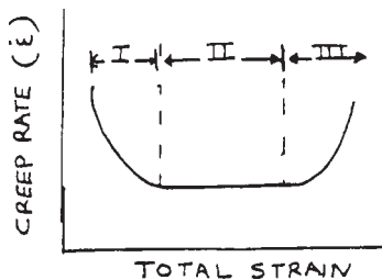
FIG. X3.1 Creep Rate
