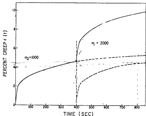
FIG. X5.1 Boltzmann Principle
